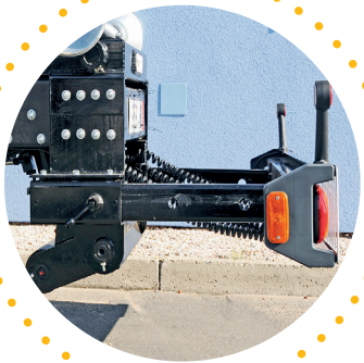
Rear extensible bumper Pare-chocs extensible
